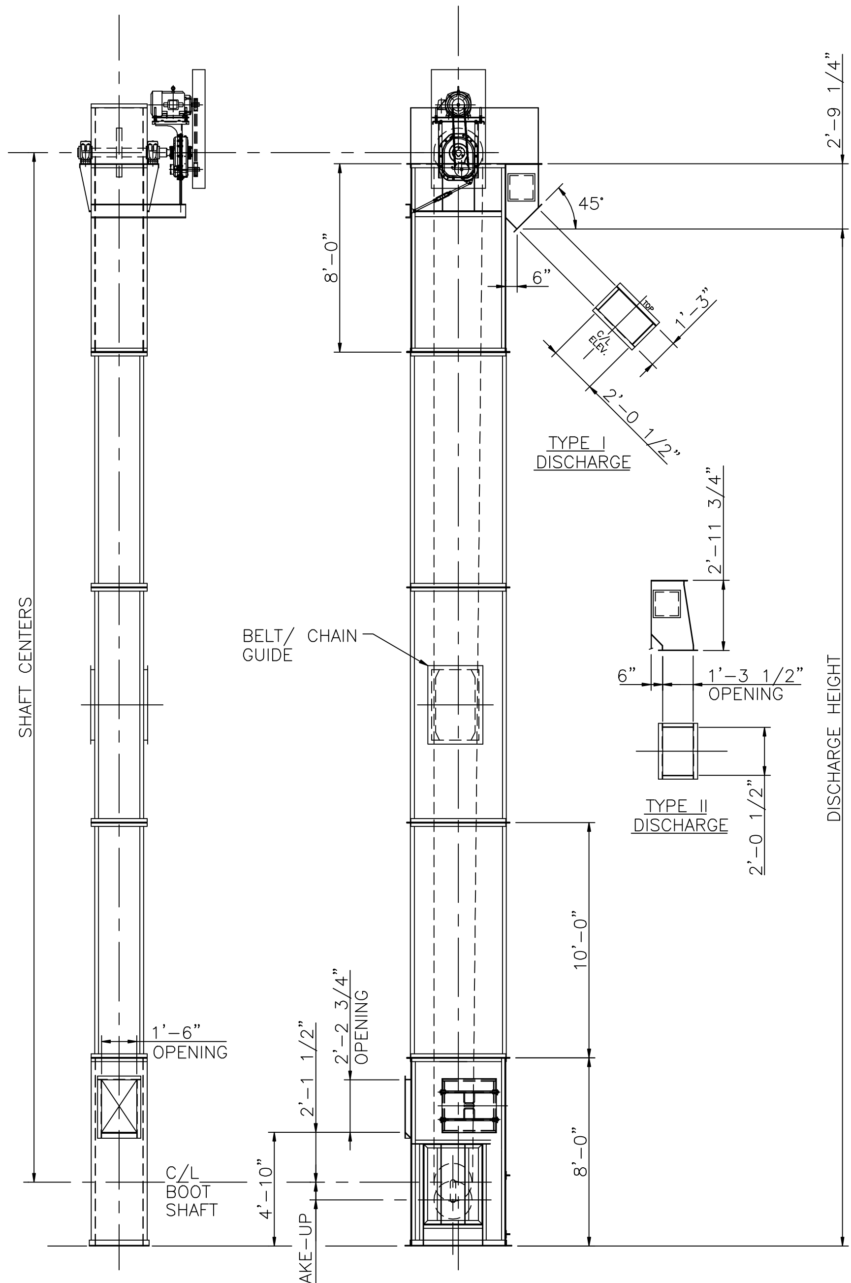
CONTINUOUS TYPE ELEVATOR 24" X 48" CASING ELEVATOR MODEL NO. CC-12724 CB-12724 CC-14724 CB-14724 CC-14824 CB-14824 CC-16824 CB-16824 CC-18824 CB-18824
