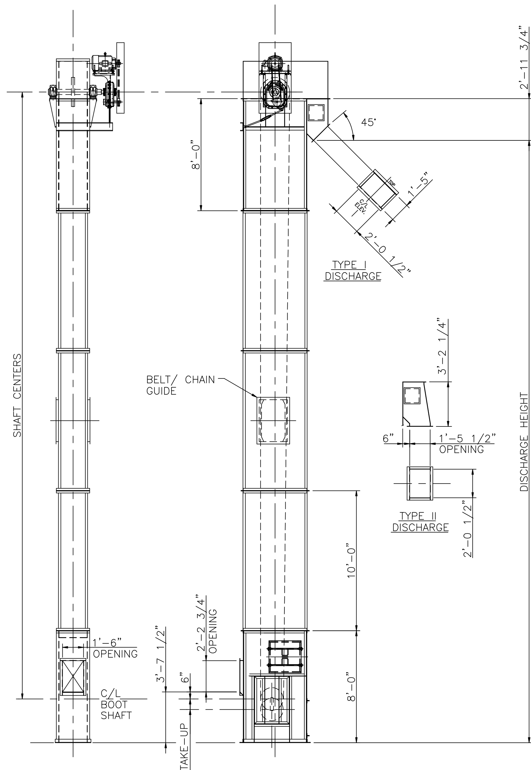
CENTRIFUGAL TYPE ELEVATOR 24" X 54" CASING ELEVATOR MODEL NO. SC-12730 SB-12730 SC-14730 SB-14730 SC-16824 SB-16824 SC-16830 SB-16830
